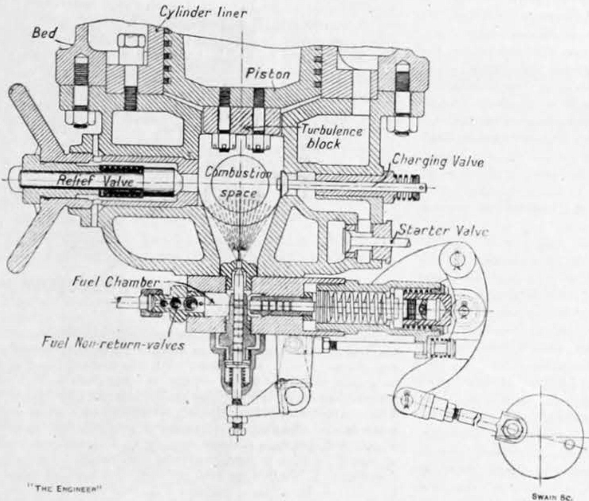
FIG. 7—FUEL INJECTION ARRANGEMENT—BLACKSTONE
