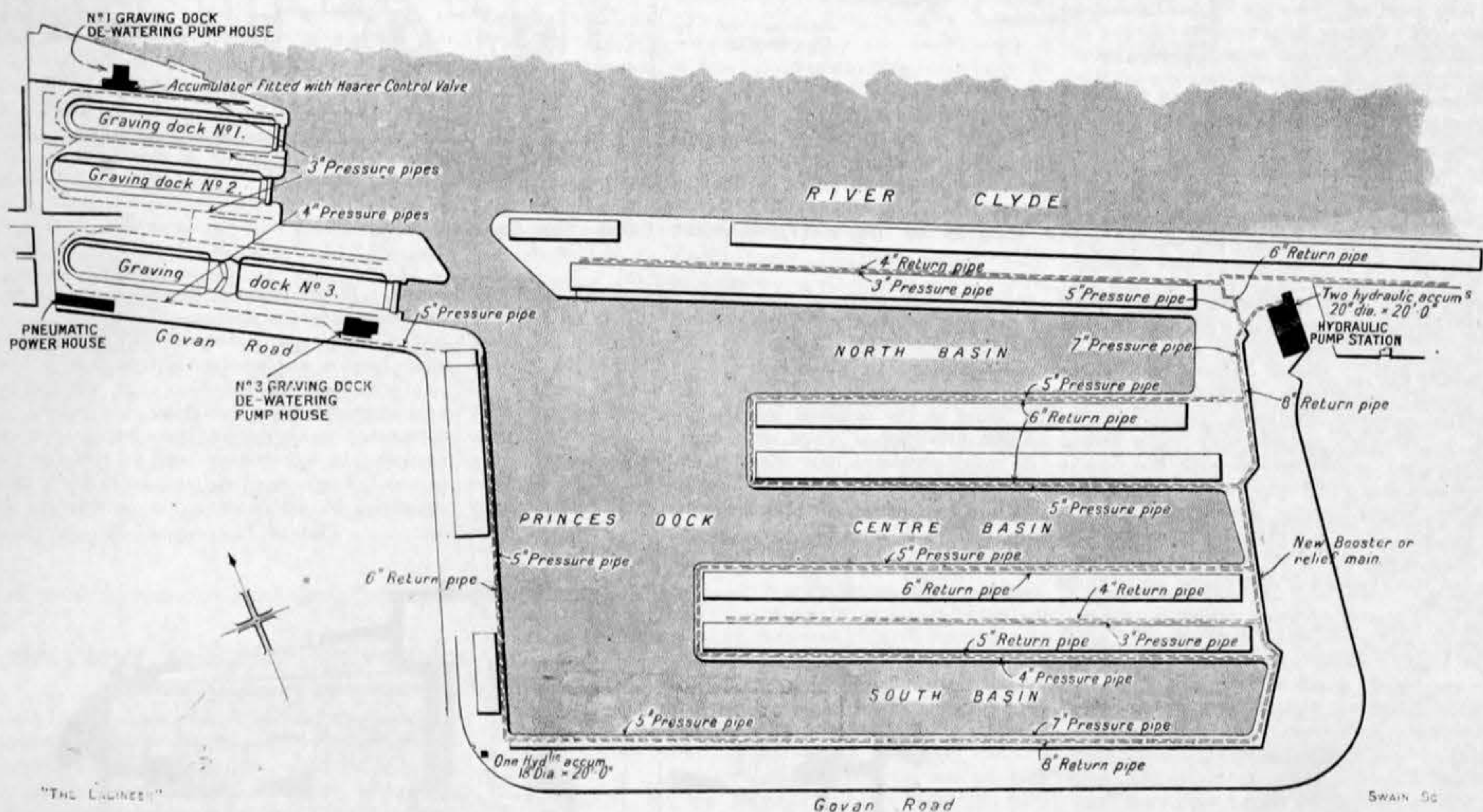
FIG. 1—PLAN SHOWING PRINCE'S DOCK AND GRAVING DOCKS NOS. 1, 2 AND 3 AND POSITIONS OF POWER HOUSES
