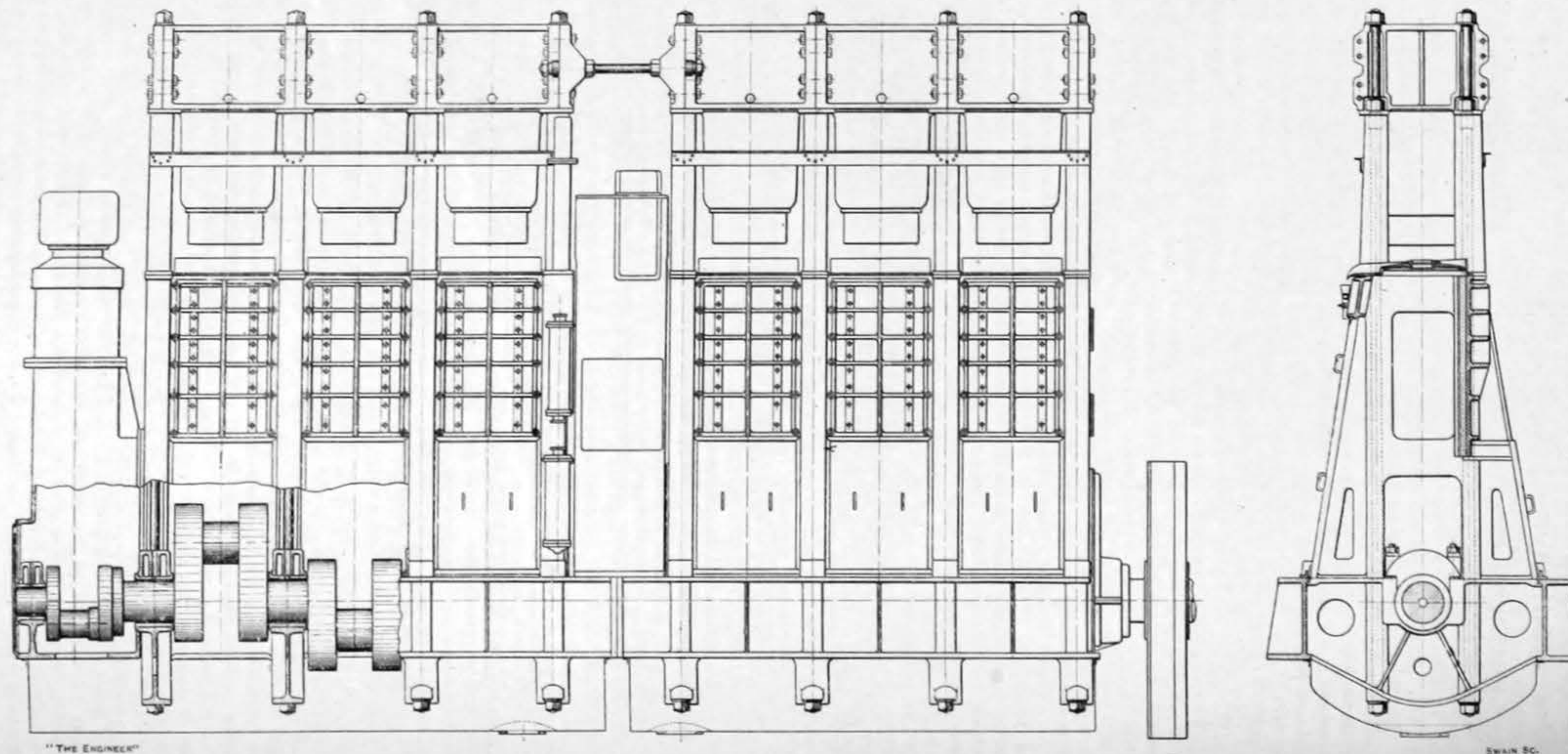
FIG. 2—GENERAL ARRANGEMENT OF SIX-CYLINDER SINGLE-ACTING ENGINE
