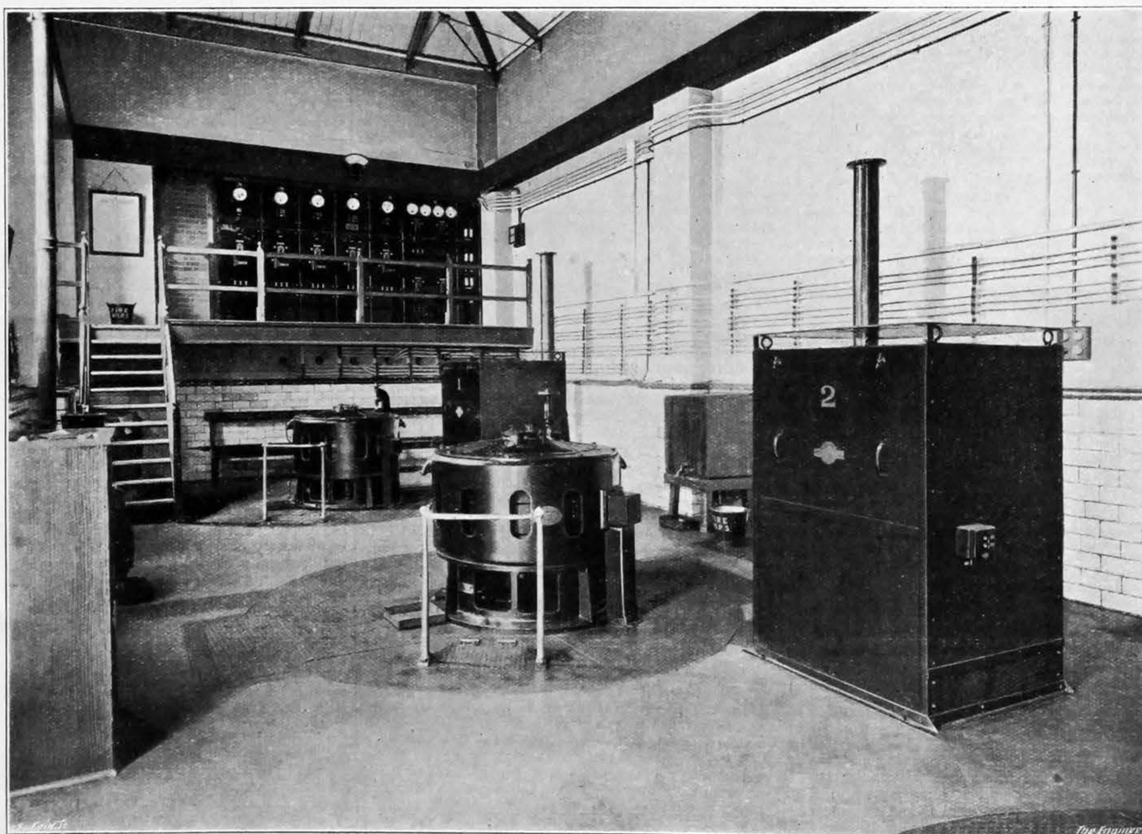
FIG. 6—INTERIOR OF PUMP HOUSE SHOWING MAIN PUMP MOTORS NOS. 1 AND 2
