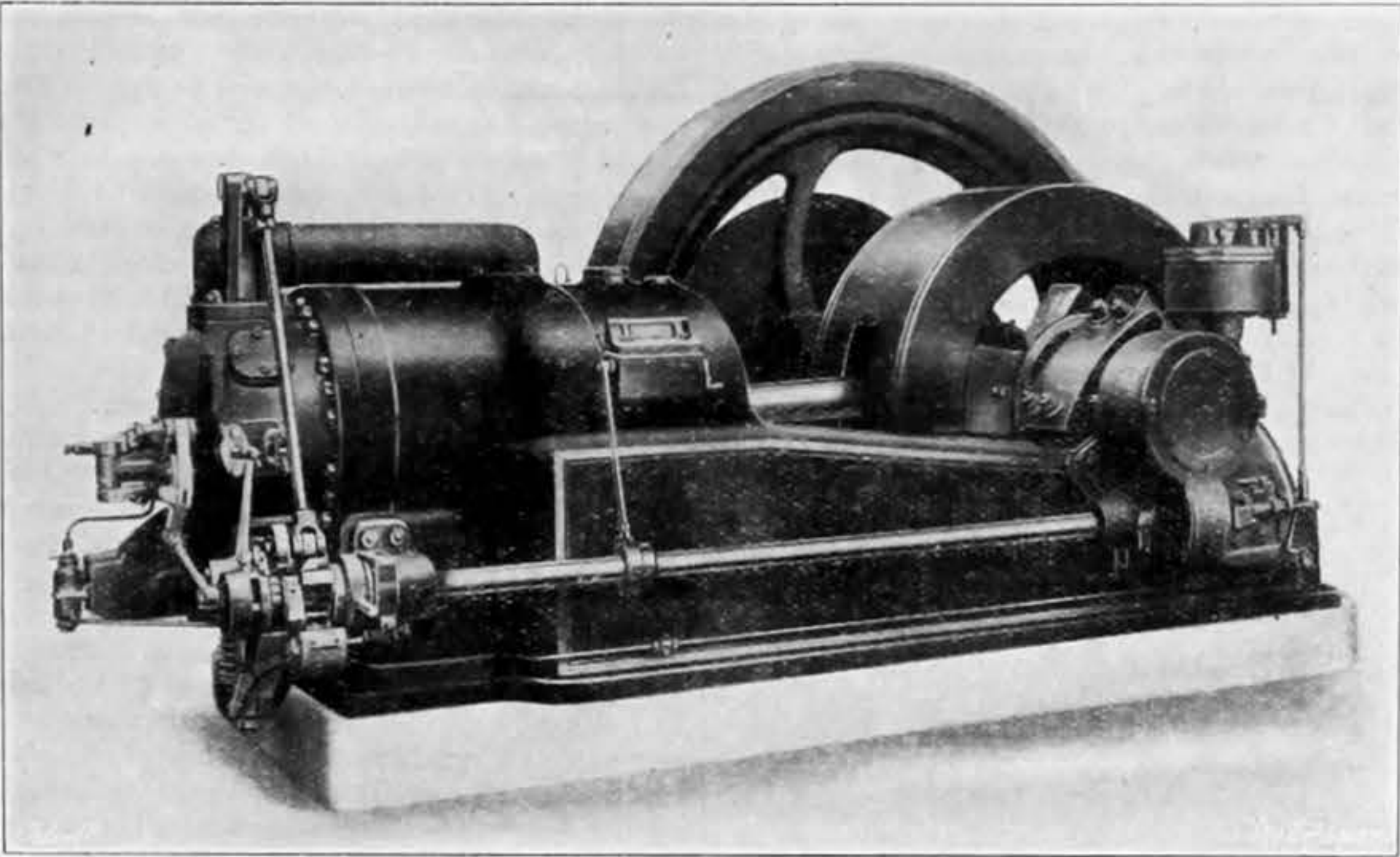
FIG. 6—55 B.H.P. OIL ENGINE—BLACKSTONE
