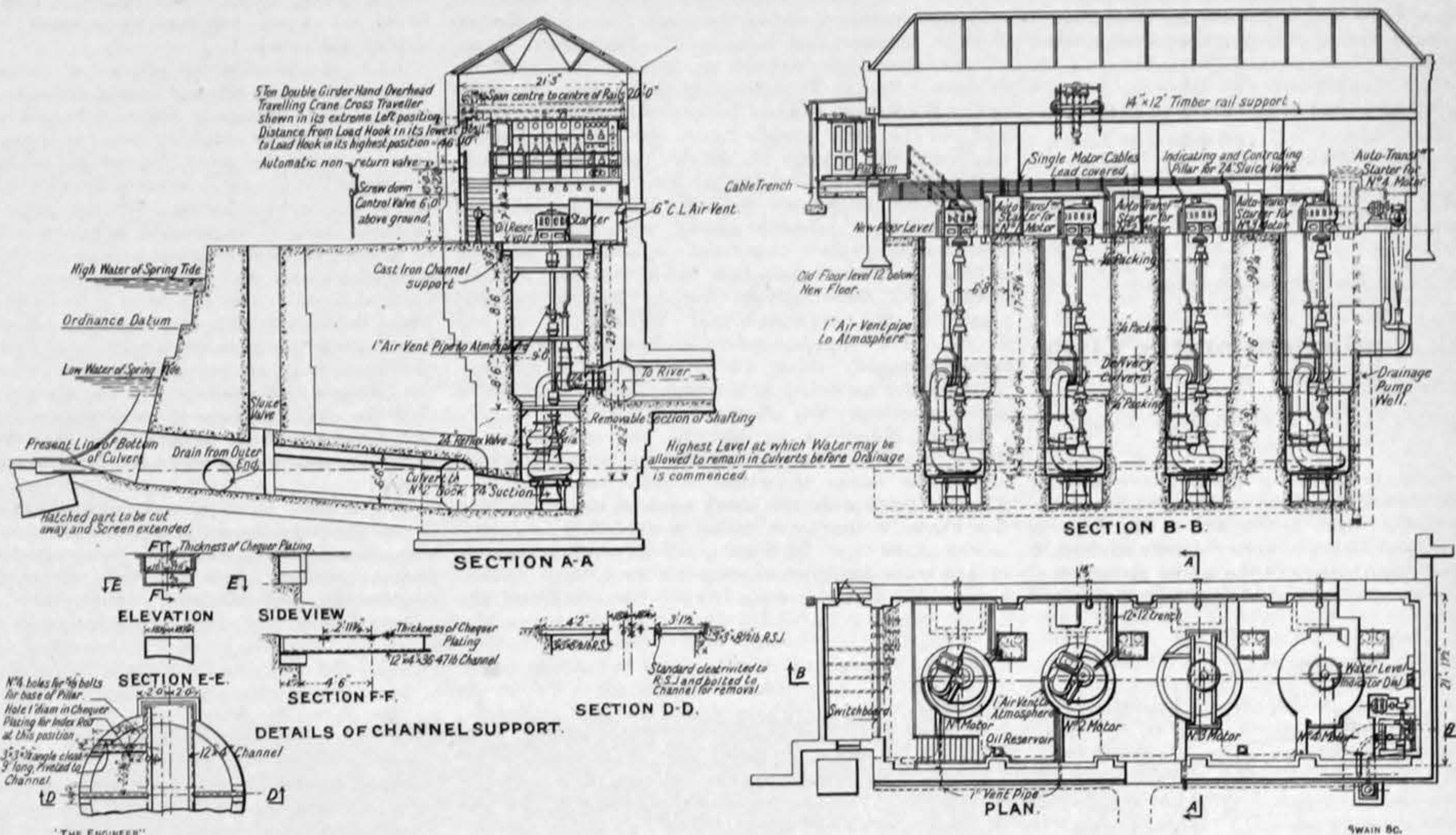
FIG. 2—PLAN AND SECTIONS OF DE-WATERING PUMP HOUSE FOR GRAVING DOCK NO. 1
