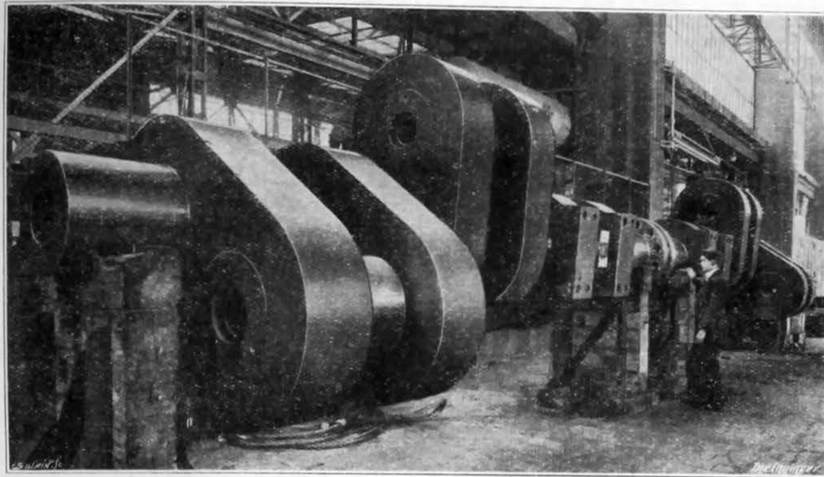
FIG. 4—CRANKSHAFT FOR 6750 S.H.P. DOUBLE-ACTING ENGINE
