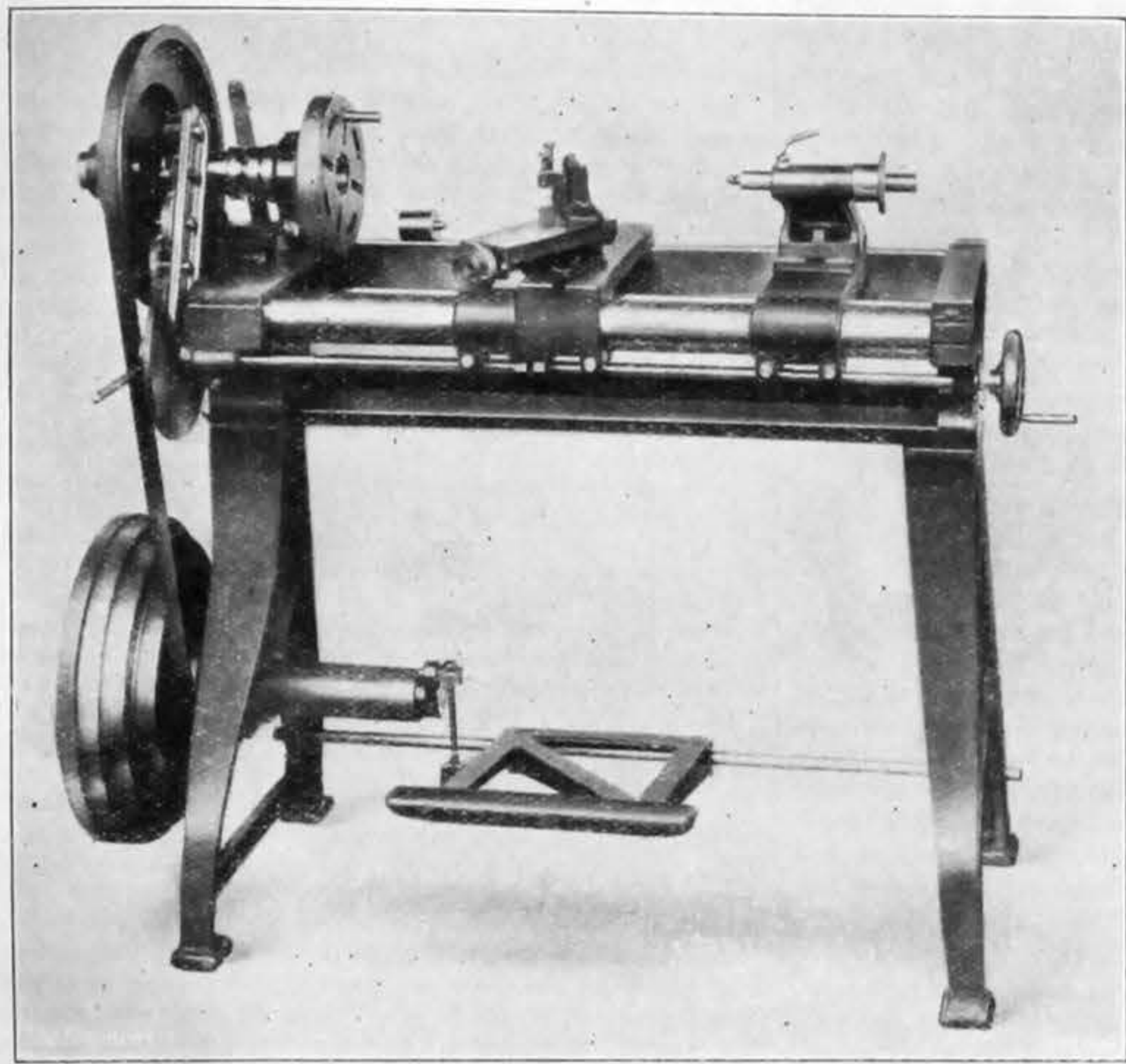
FIG. 10—SCREW CUTTING LATHE—EXE ENGINEERING CO.
