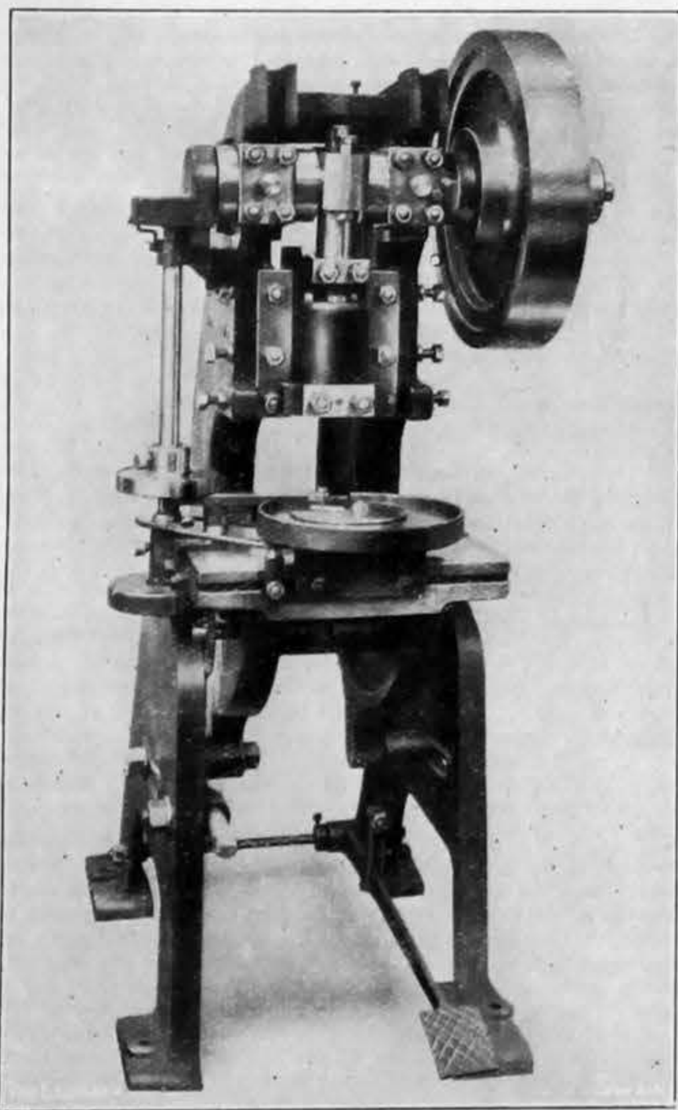
FIG. 12—INCLINABLE PRESS WITH FRICTION FEED
