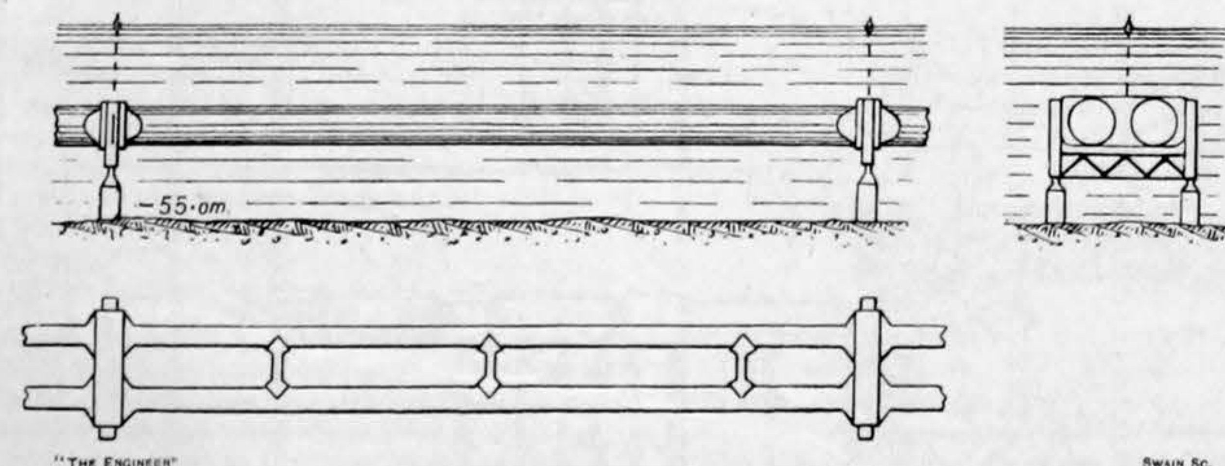
FIG. 1—PART PLAN AND ELEVATION, AND CROSS SECTION OF PROPOSED TUBULAR RAILWAY
