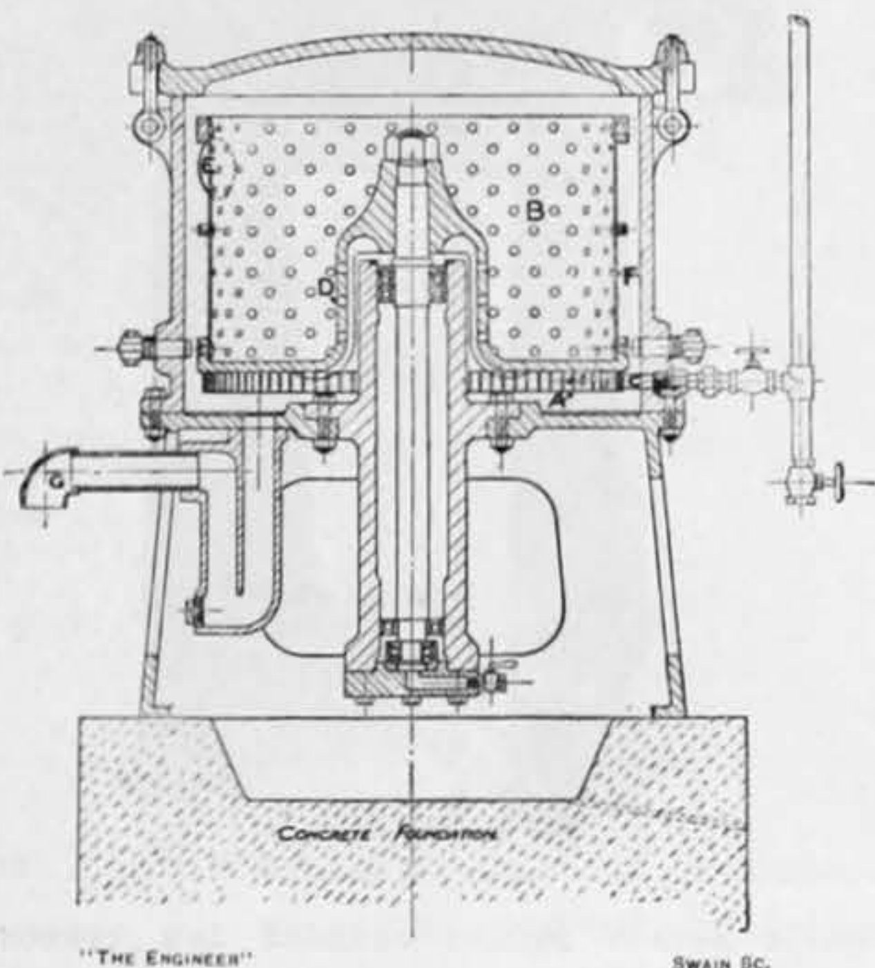
FIG. 15—OIL SEPARATOR—INDUSTRIAL WASTE ELIMINATORS
