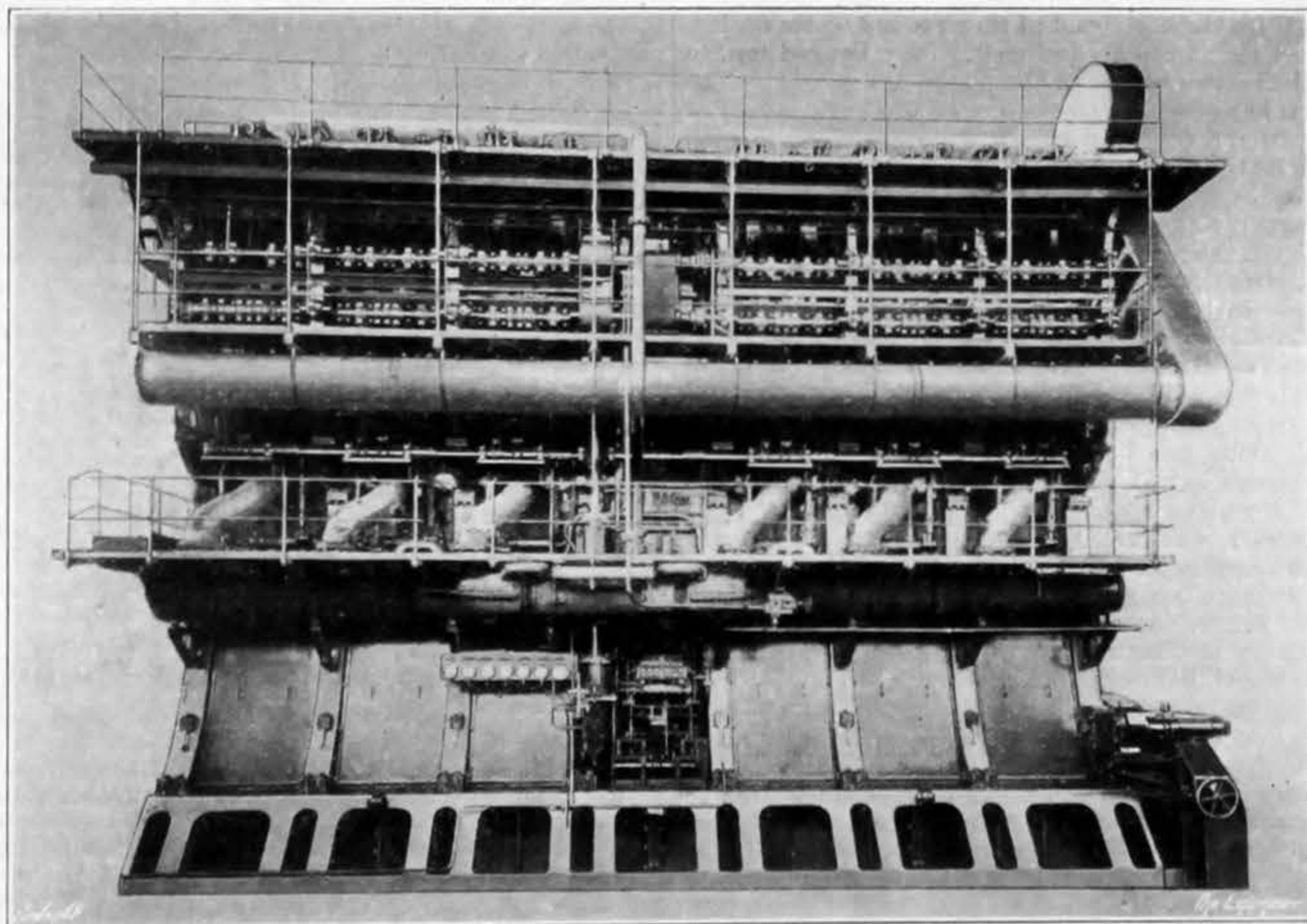
FIG. 5—6750 S.H.P. DOUBLE-ACTING ENGINE FOR THE MOTOR LINER GRIPSHOLM
