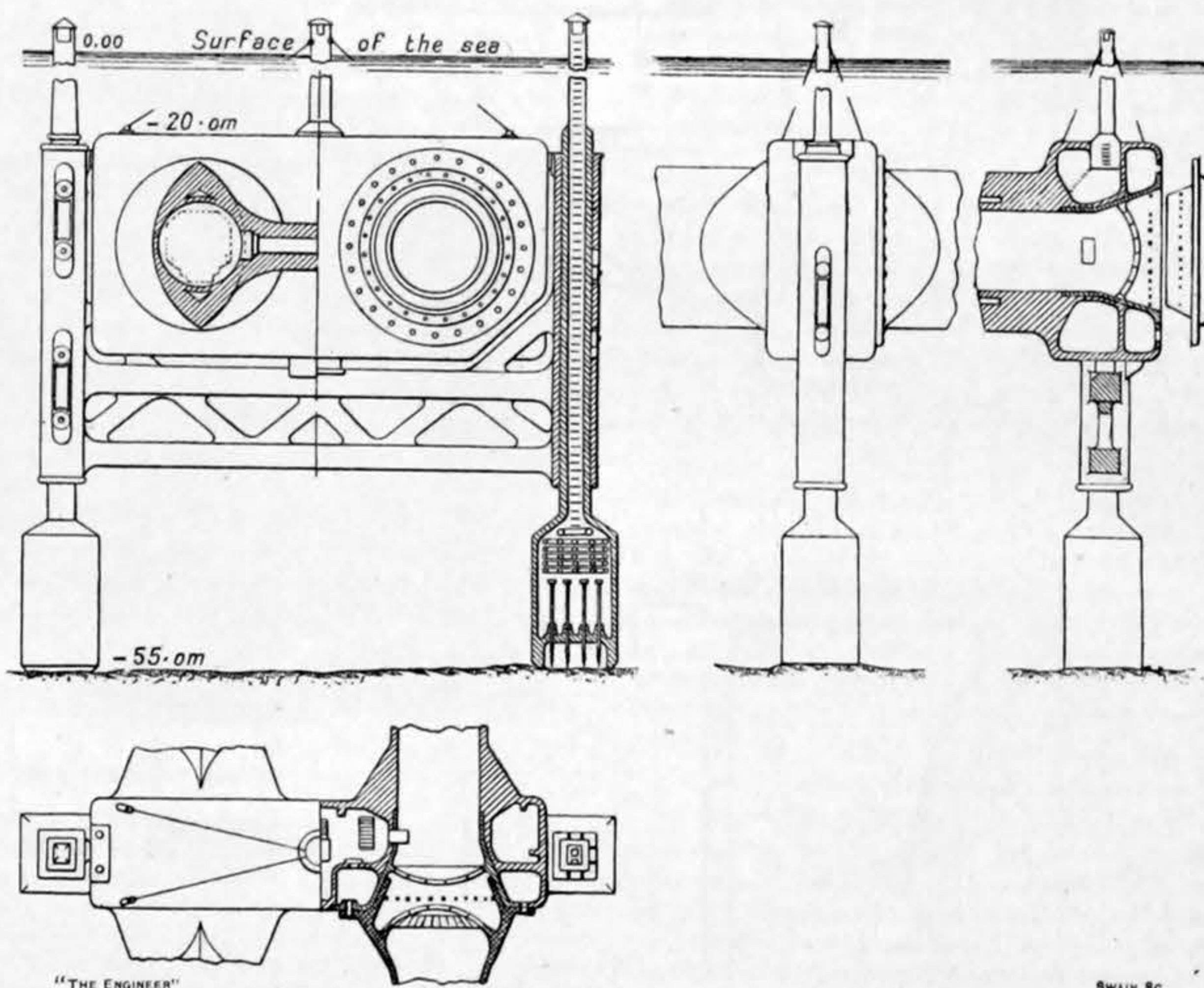
FIG. 2—ARRANGEMENT OF PIERS, TUBES AND JOINTS OF TUBULAR RAILWAY
