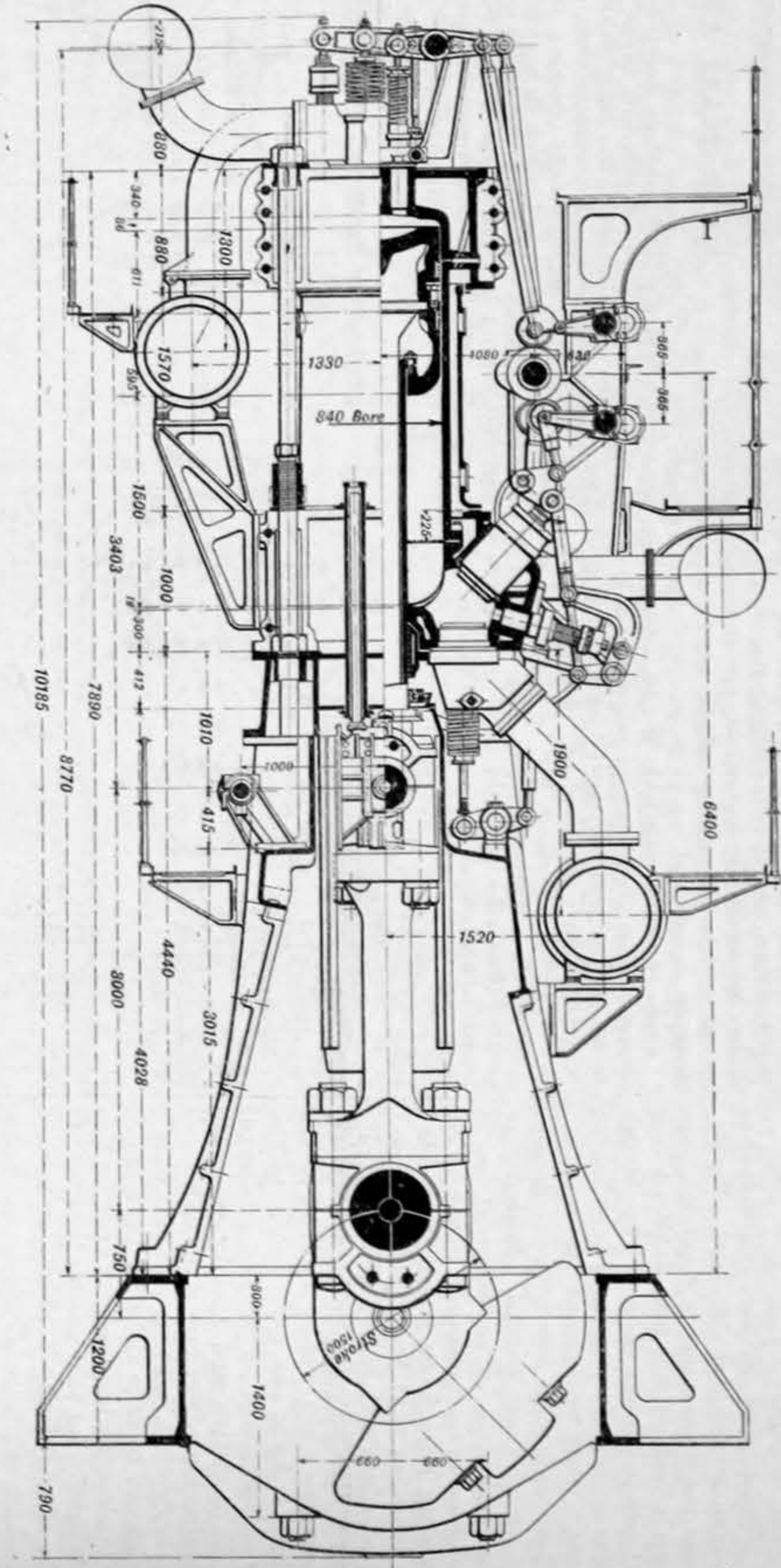
FIG. 3—SECTIONS OF DOUBLE-ACTING ENGINE
