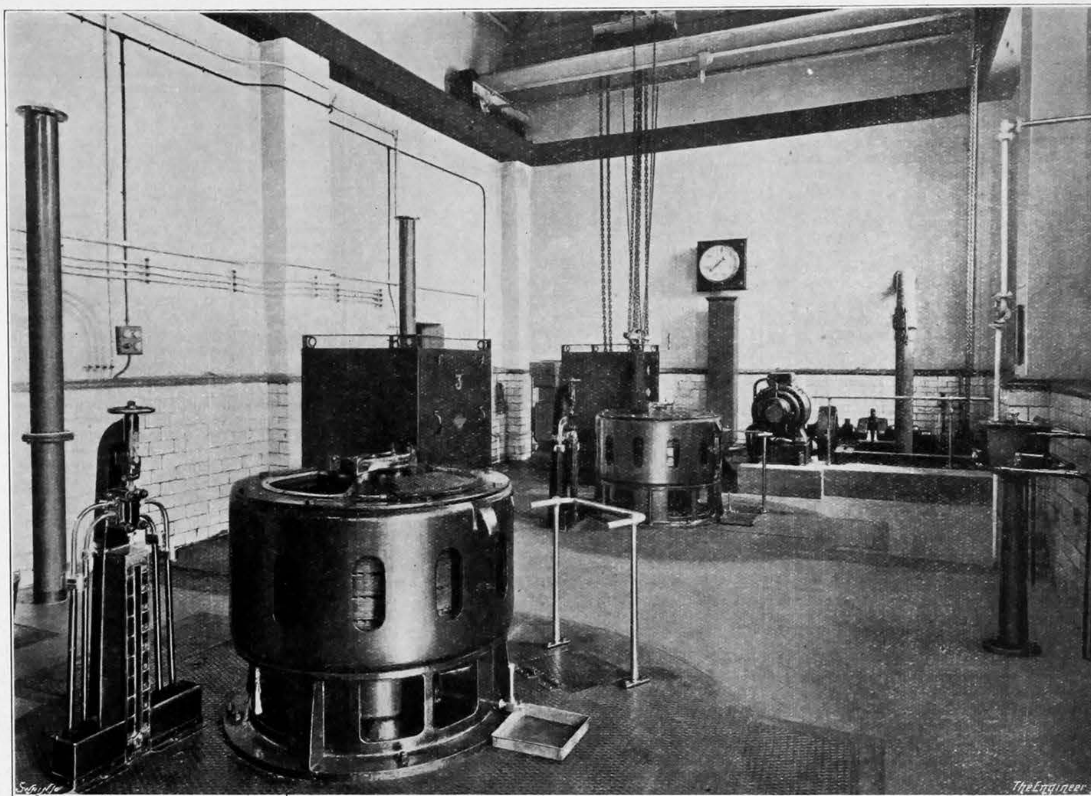
FIG. 5—INTERIOR OF PUMP HOUSE SHOWING MAIN PUMP MOTORS NOS. 3 AND 4
