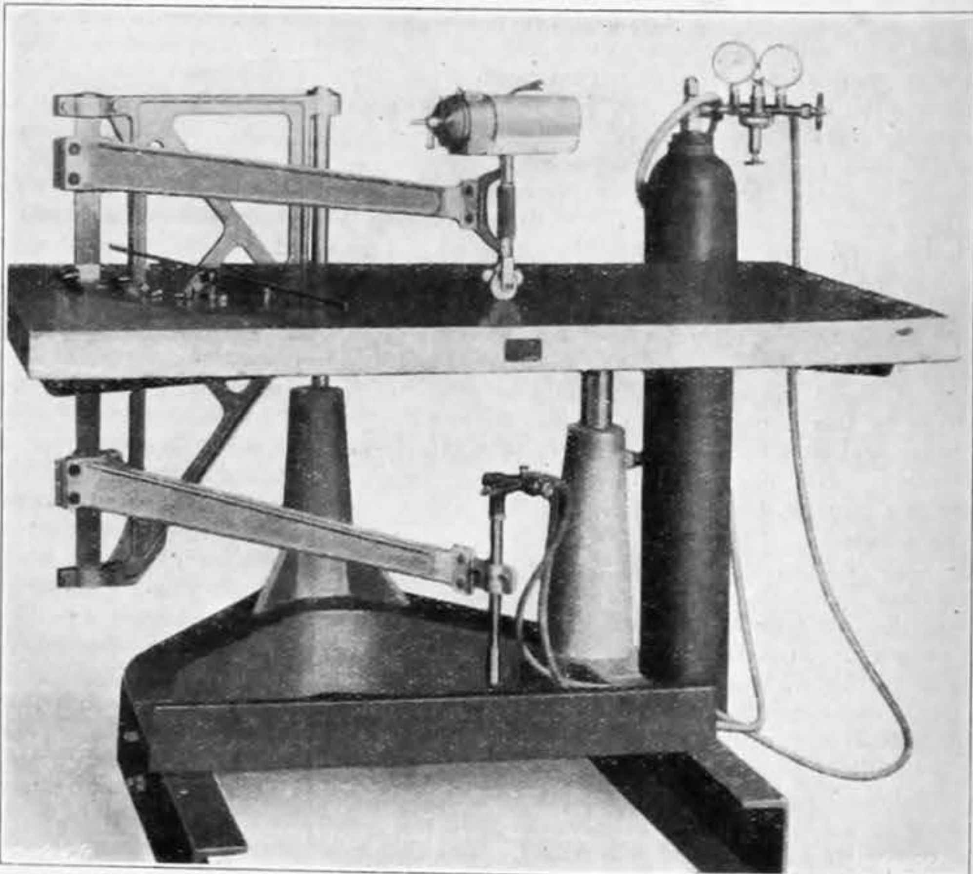
FIG. 8—OXYGEN CUTTING PLANT—HANCOCK
