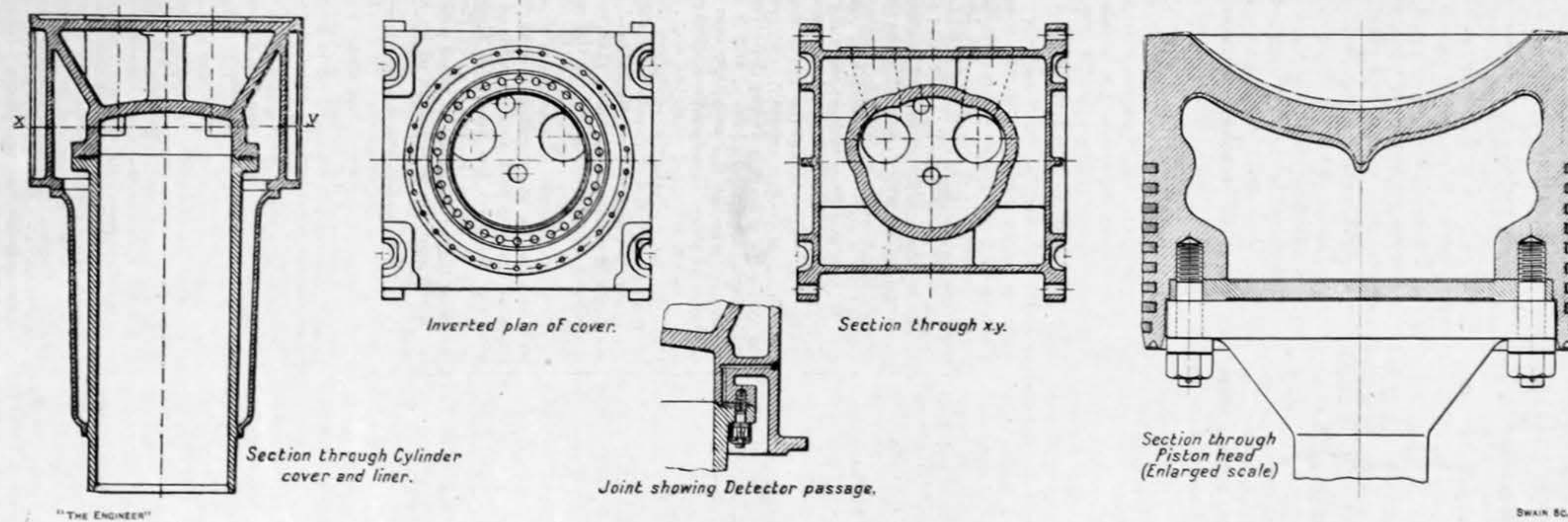
FIG. 1—DETAILS OF CYLINDER COVER, LINER AND PISTON FOR SINGLE-ACTING ENGINES
