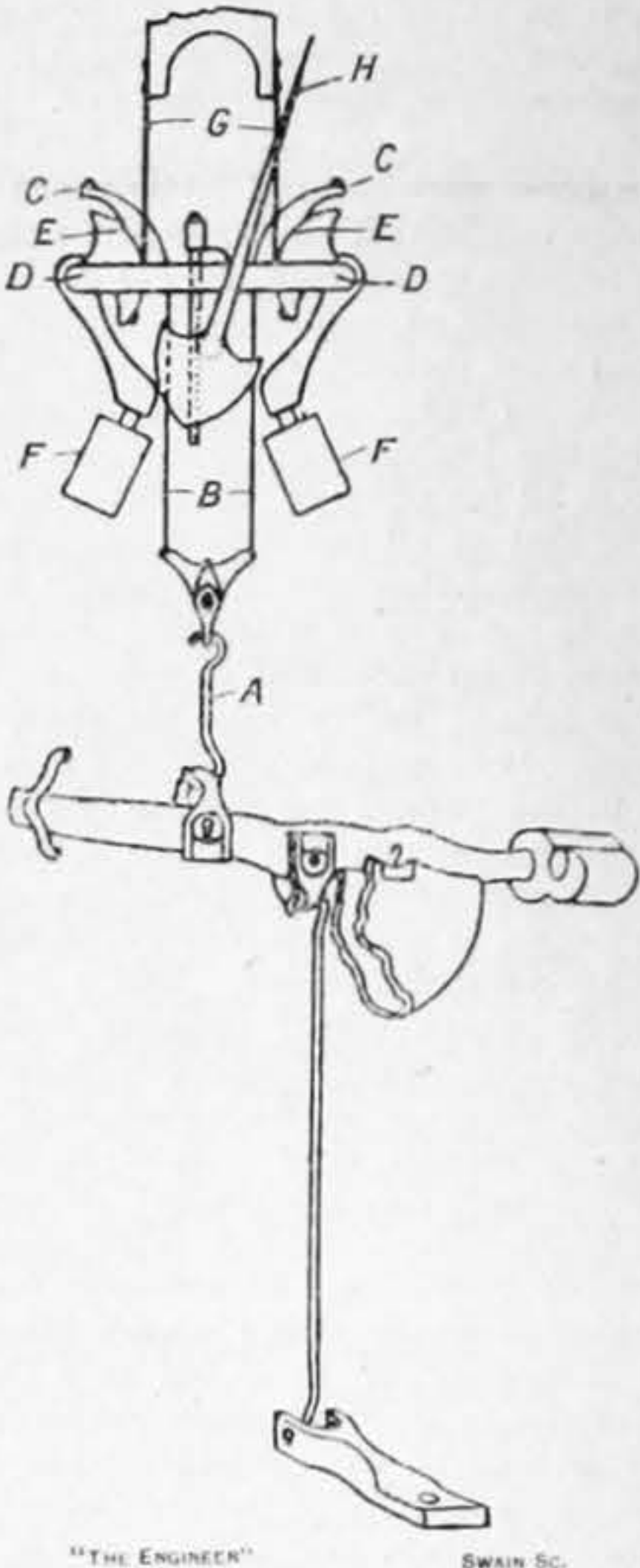
FIG. 9—MECHANISM OF WEIGHING MACHINE—AVERY
