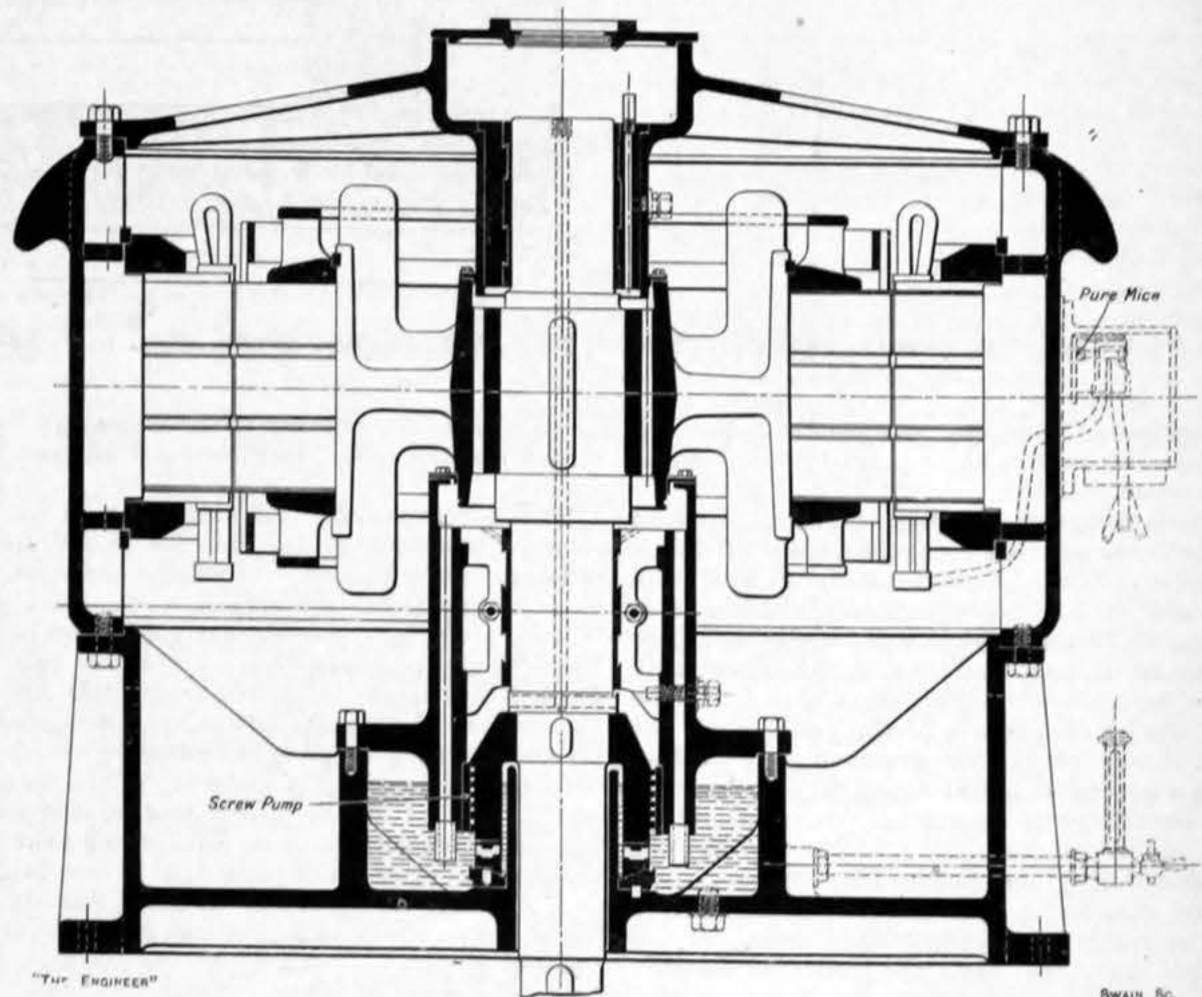
FIG. 4—SECTION OF MOTOR SHOWING SCREW OIL CIRCULATING PUMP
