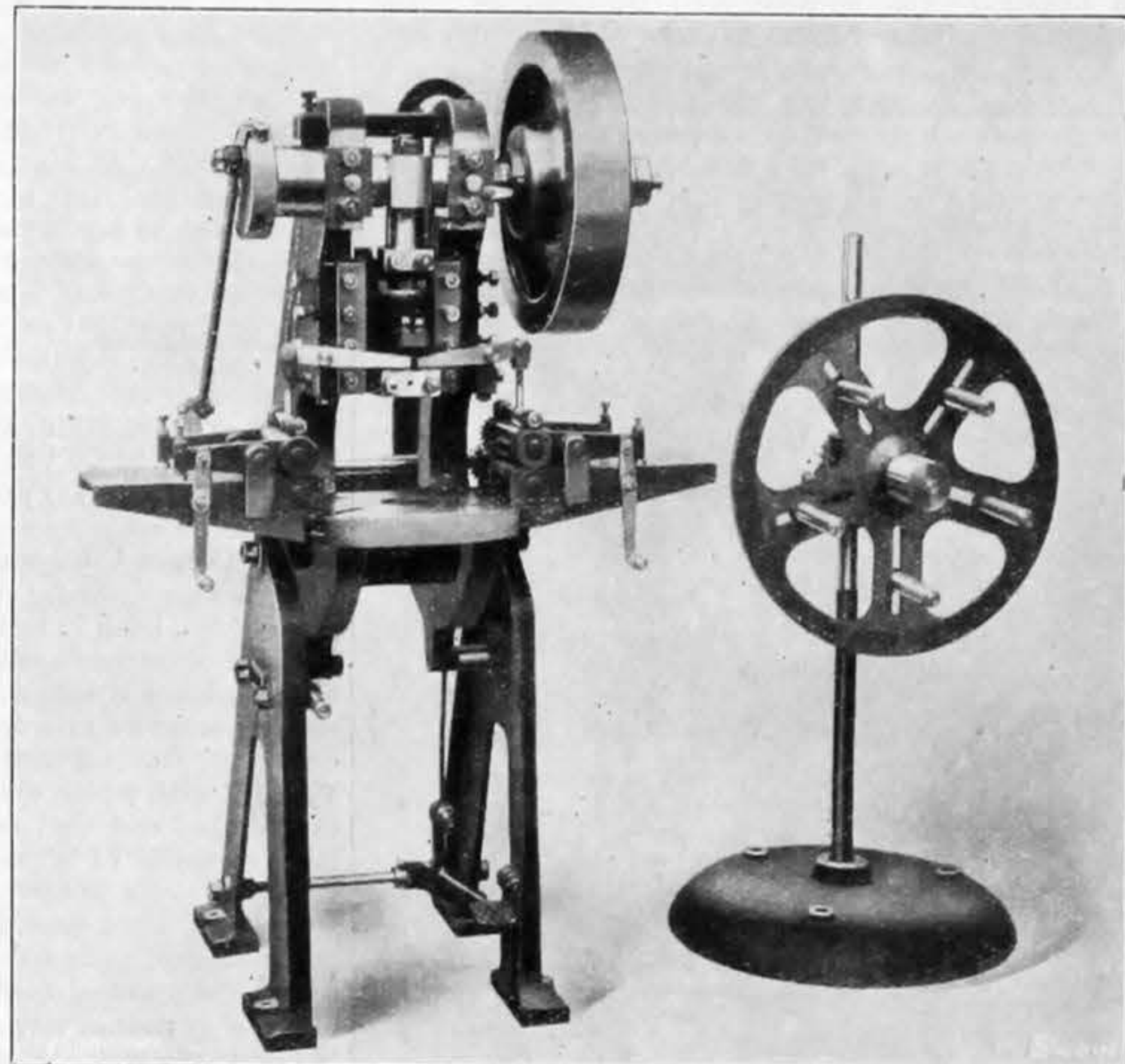
FIG. 11—INCLINABLE PRESS WITH DOUBLE ROLL FEED—BRADLEY &amp; TURTON
