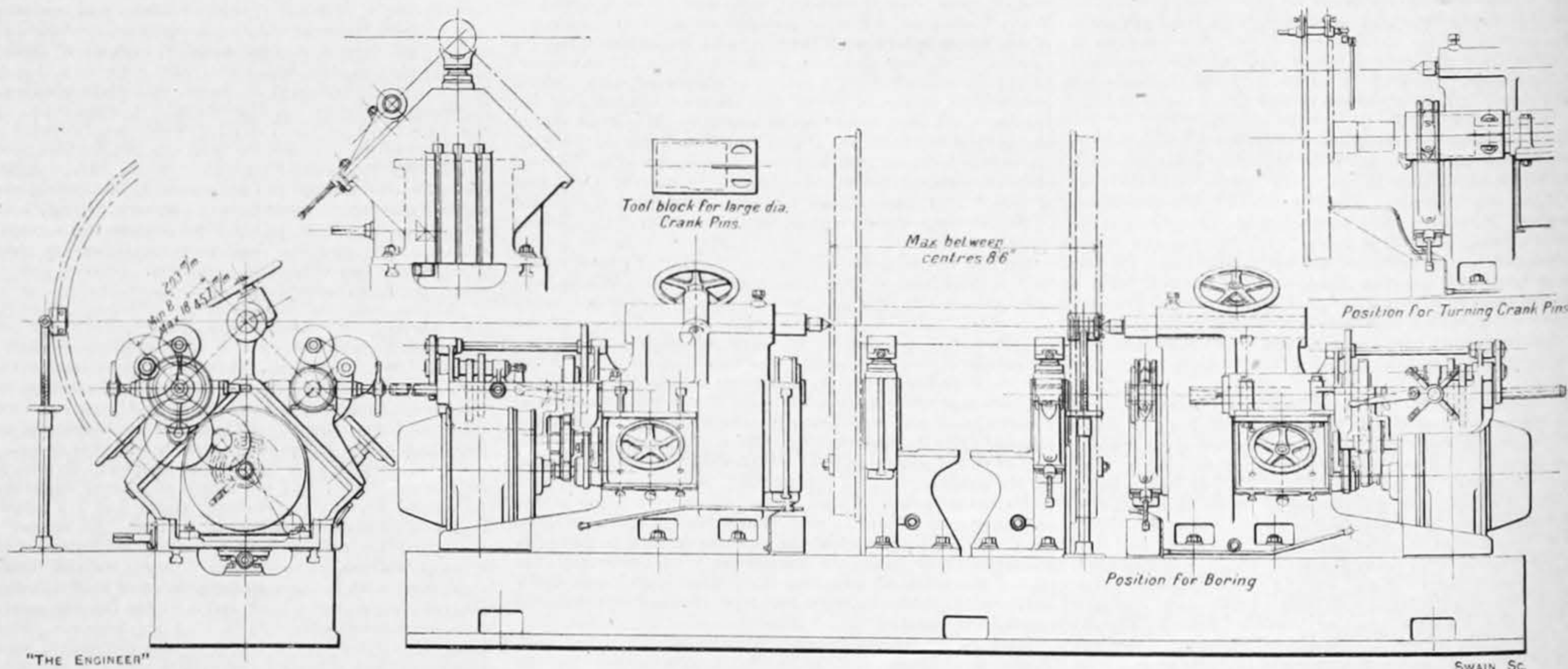
ARRANGEMENT OF LOCOMOTIVE WHEEL QUARTERING MACHINE
